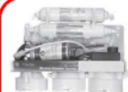
Components with filter cartridges AICRO, AIMRO, PUMP ®
